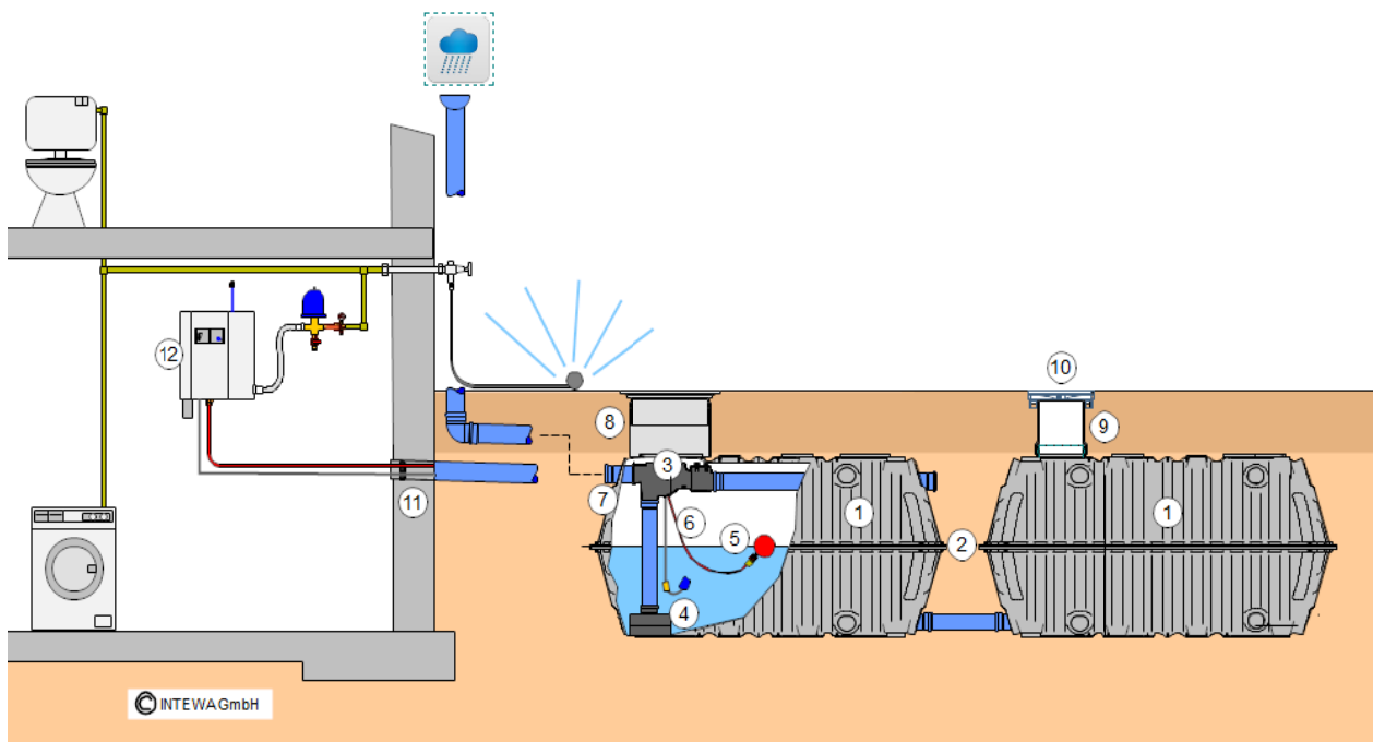
Figure 7: Example system Home application
