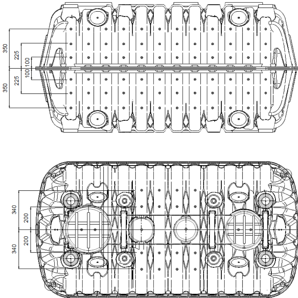
Figure 9: Drilling plan for side and bottom area
