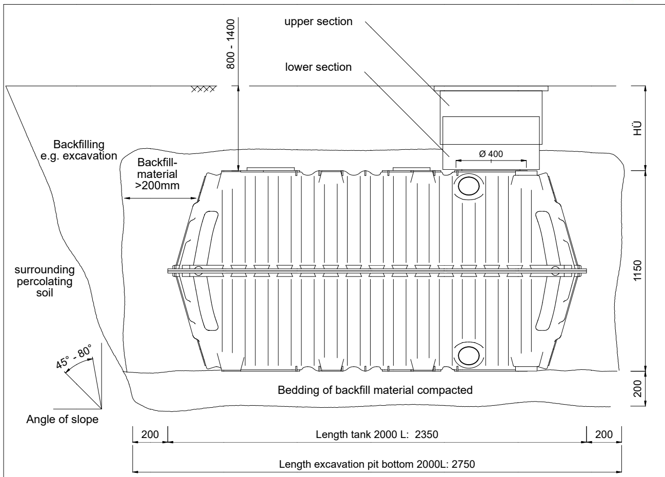
Figure 3: Installation trafficable version with telescopic dome
