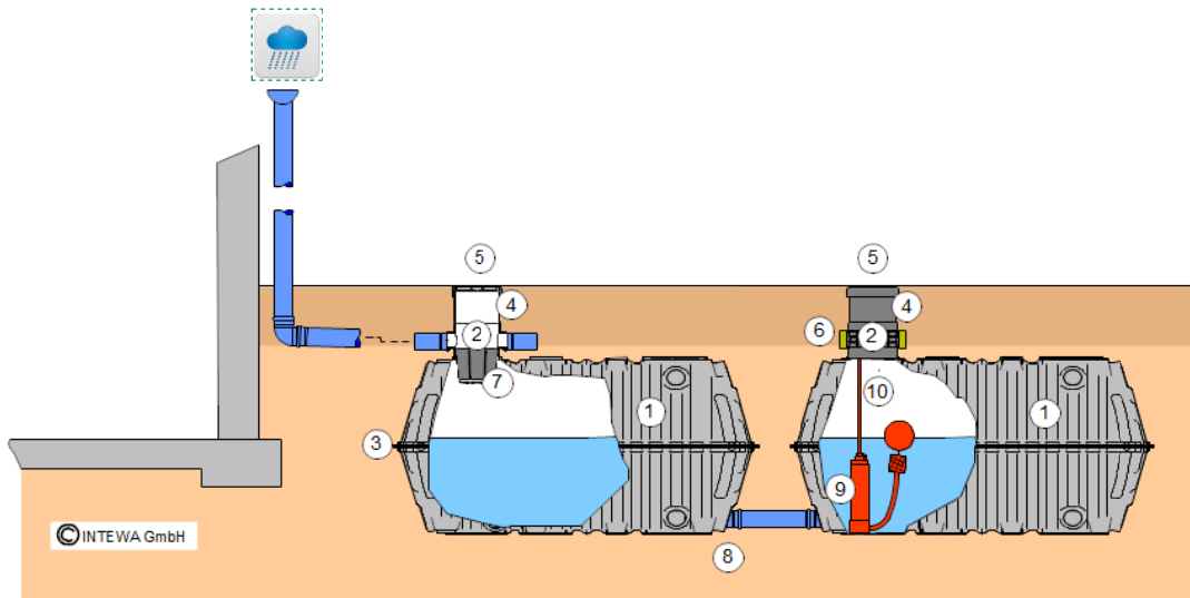
Figure 6: Example system Garden system 4000 liters
