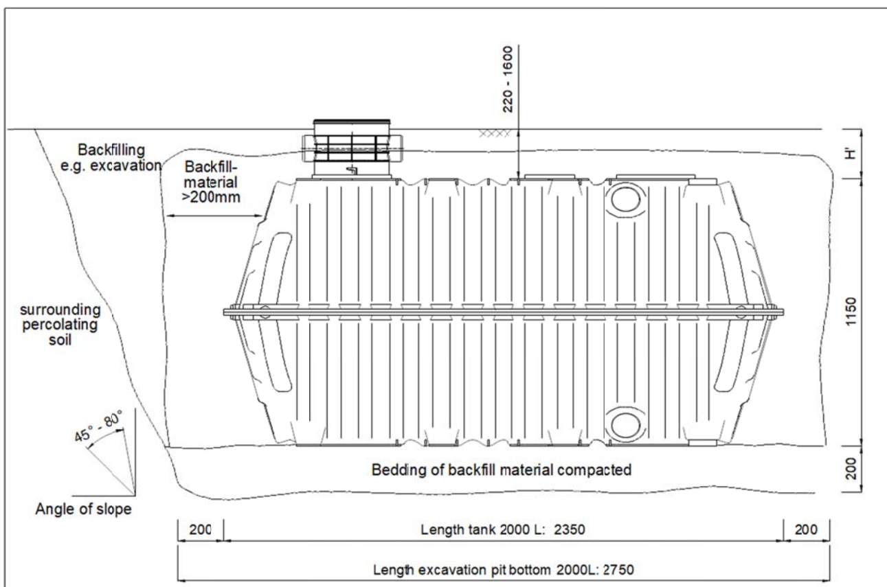
Figure 2: Installation walkable version
