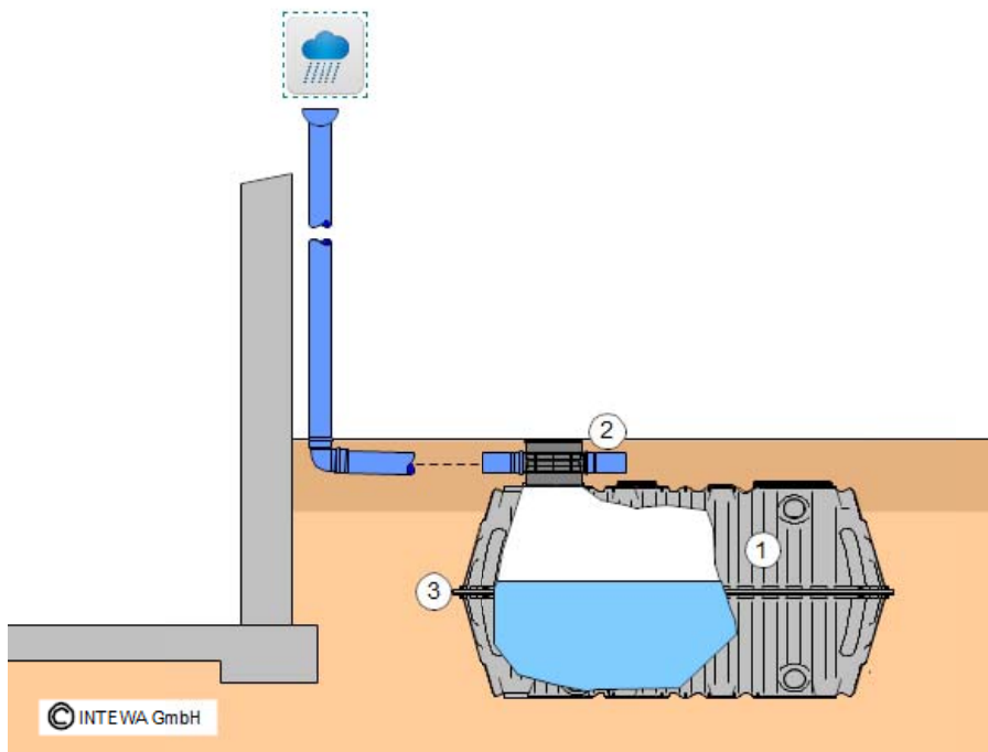
Figure 5: Example system Garden system 2000 liters
