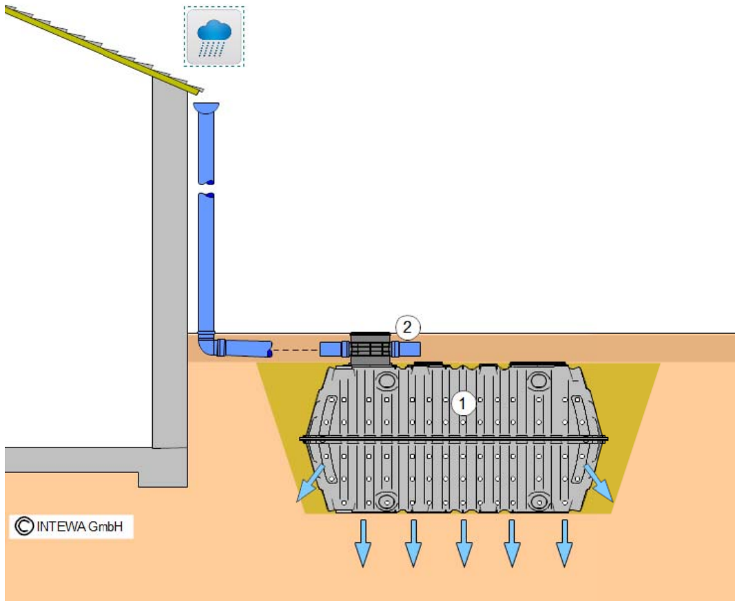
Figure 8: Example system infiltration 2000 liters
