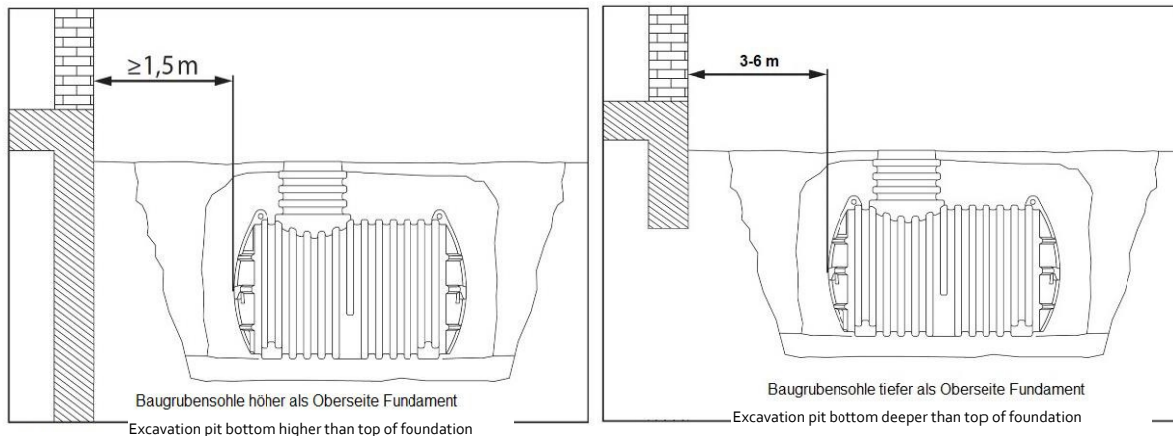
Figure 4: Distance to the building
