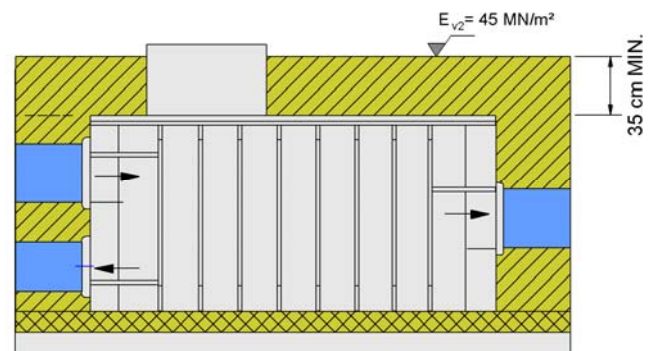
Fig. 11: Backfilling up to 35 cm above tank shoulder
