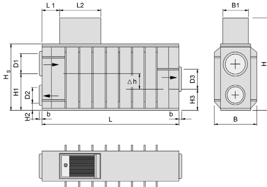
Fig. 3: Dimensions of PURAIN-HD 200
