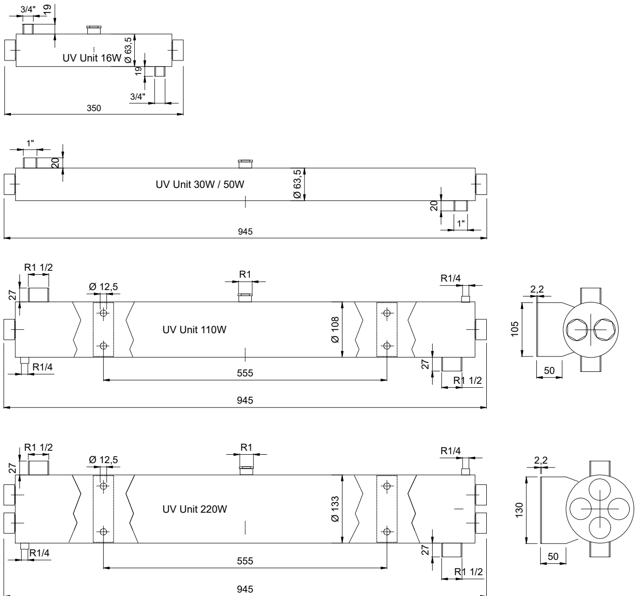
Figure: Dimensions of the UV-I-UNITS
